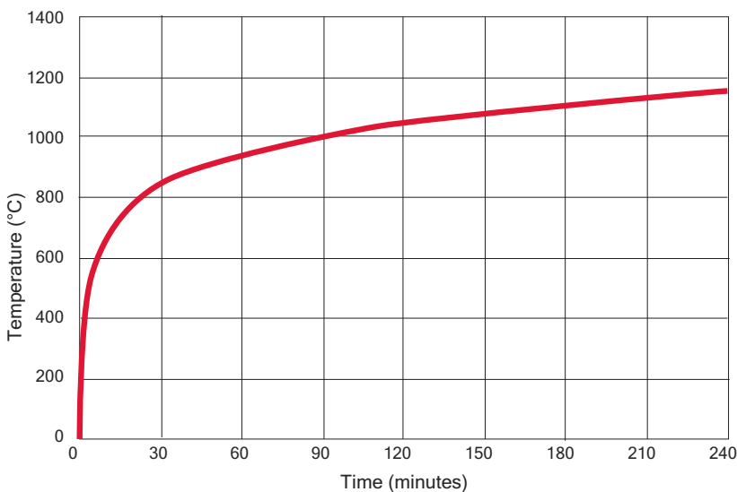
Standard Time/Temp. Curve (4 hours) As specified in EN 1363-1
