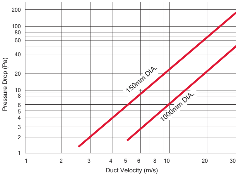
Pressure Drop Graph Type B, Type C and Type O Maximum unrestricted airflow Velocity range 0 to 30 m/s
